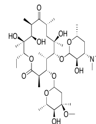
Chemical structure of Erythromycin
