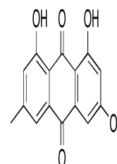
Chemical structure of Emodin
