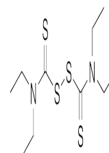
Chemical structure of Disulfiram
