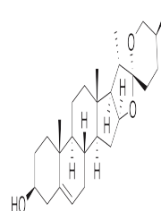
Chemical structure of Diosgenin
