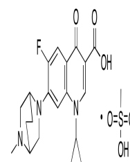
Chemical structure of Danofloxacin Mesylate
