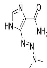
Chemical structure of Dacarbazine
