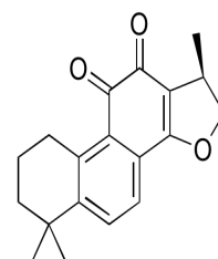
Chemical structure of Cryptotanshinone
