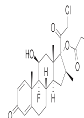
Chemical structure of Clobetasol Propion...
