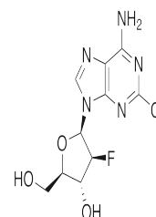
Chemical structure of Clofarabine
