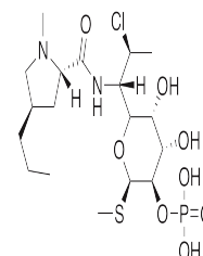
Chemical structure of Clindamycin Phosph...
