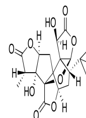
Chemical structure of Ginkgolide A
