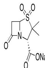
Chemical structure of Sulbactam Sodium
