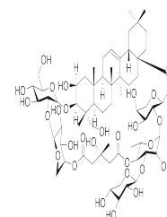
Chemical structure of Tubeimoside I
