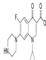
Chemical structure of Ciprofloxacin
