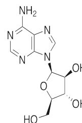
Chemical structure of Vidarabine
