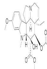
Chemical structure of Vindoline
