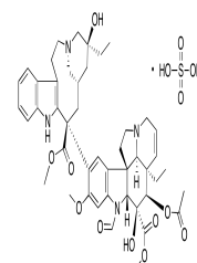
Chemical structure of Vincristine Sulfate...
