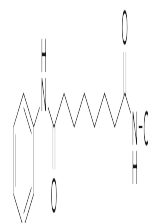
Chemical structure of Vorinostat
