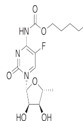
Chemical structure of Capecitabine
