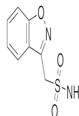
Chemical structure of Zonisamide
