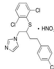
Chemical structure of Butoconazole Nitra...
