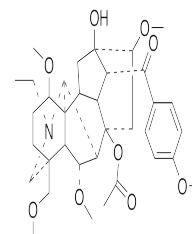
Chemical structure of Bulleyaconitine A
