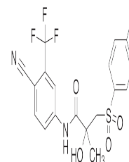
Chemical structure of Bicalutamide
