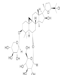
Chemical structure of Astragaloside IV
