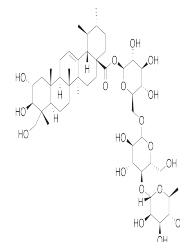
Chemical structure of Asiaticoside
