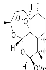
Chemical structure of Artemether
