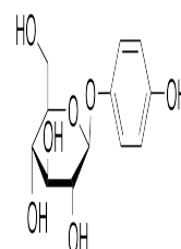
Chemical structure of Arbutin
