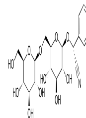
Chemical structure of Amygdalin
