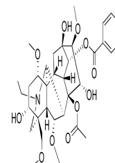
Chemical structure of Aconitine
