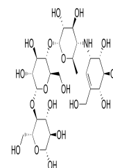
Chemical structure of Acarbose
