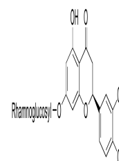
Chemical structure of Hesperidin
