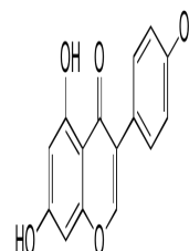
Chemical structure of Genistein
