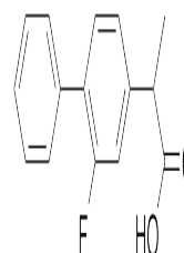
Chemical structure of Flurbiprofen
