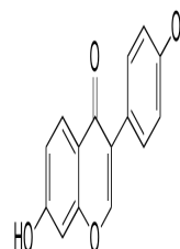
Chemical structure of Daidzein
