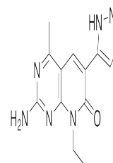
Chemical structure of XL-765
