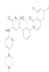
Chemical structure of RN-486
