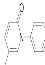
Chemical structure of Pirfenidone
