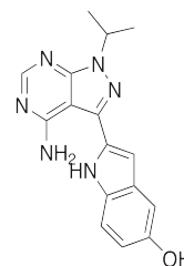
Chemical structure of PP-242
