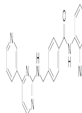
Chemical structure of MGCD-0103
