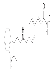
Chemical structure of LBH-589
