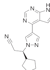
Chemical structure of INCB018424
