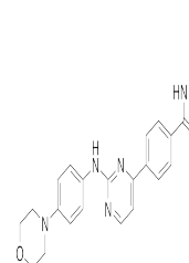
Chemical structure of CYT-387
