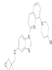
Chemical structure of Crenolanib
