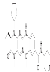
Chemical structure of BI-2536
