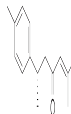
Chemical structure of (S)-ar-Turmerone
