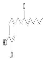
Chemical structure of Shogaol
