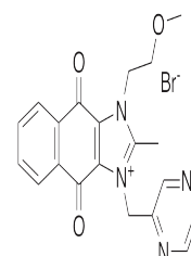
Chemical structure of YM-155
