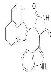
Chemical structure of Tivantinib
