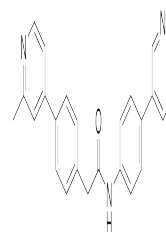
Chemical structure of C59
