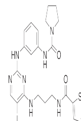
Chemical structure of BX-795
